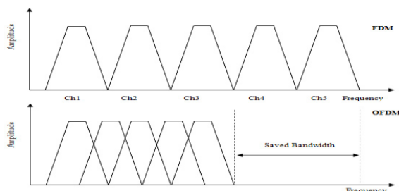
Fig.1 Spectra of FDM and OFDM for Web 3.0 Networks
