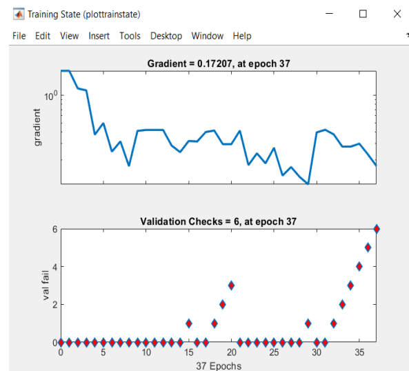
Fig 8: Training States
