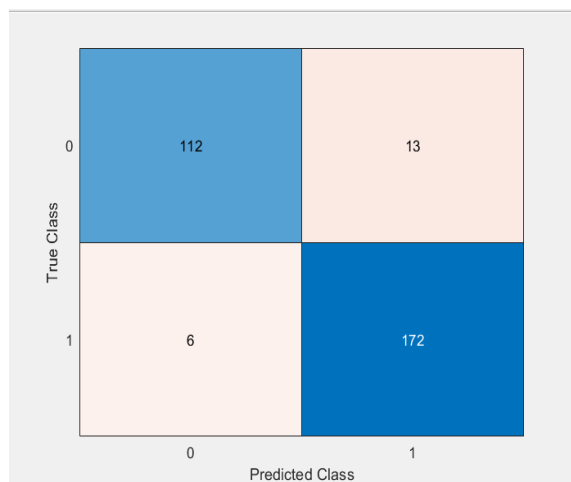
Fig 11: Confusion Matrix
