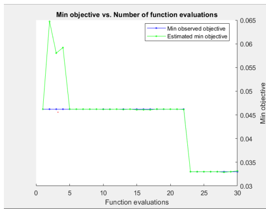
Fig 9: Function Evaluations.
