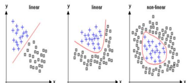
Fig 2: Linear and Non-Linear Regression fitting.
