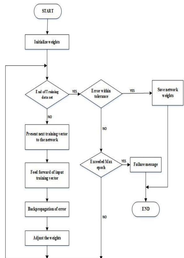
Fig.2 Flowchart of Back Propagation
