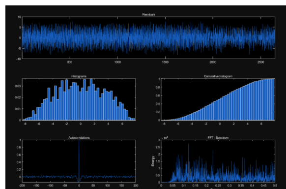
Fig.6 Multi-Resolution Analysis
