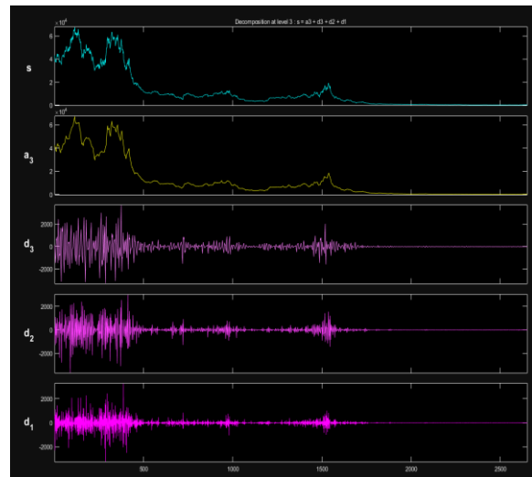
Fig.4 Haar Decomposition at Level 3
