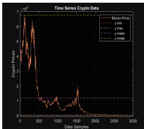
Fig.3 Original Bitcoin Price
