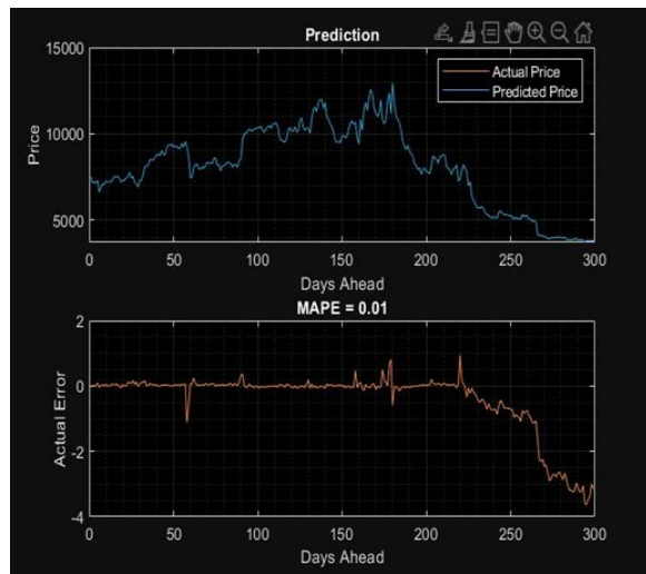
Fig.8 Predicted and Actual Crypto Behavior
