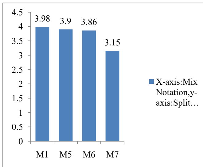
Graph 4.10: Variation of Split tensile strength with fixed Ground Granulated Blast Furnace Slag (GGBS) %(10%) vs variation of steel fibers % at the end of 28days
