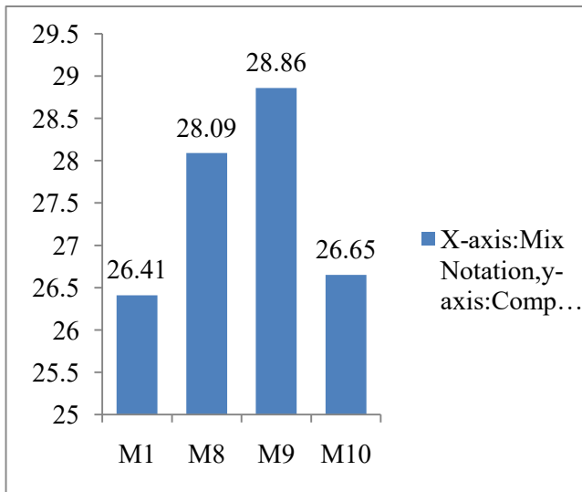
Graphs 4.6: Variation of Compression strength with fixed Ground Granulated Blast Furnace Slag (GGBS) % (10%) vs. variation of carbon fiber % at the end of 28days
