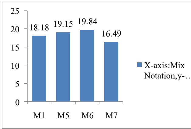
Graphs 4.3: Variation of Compression strength with fixed Ground Granulated Blast Furnace Slag (GGBS) %(10%) vs variation of steel fiber %.at the end of 7days
