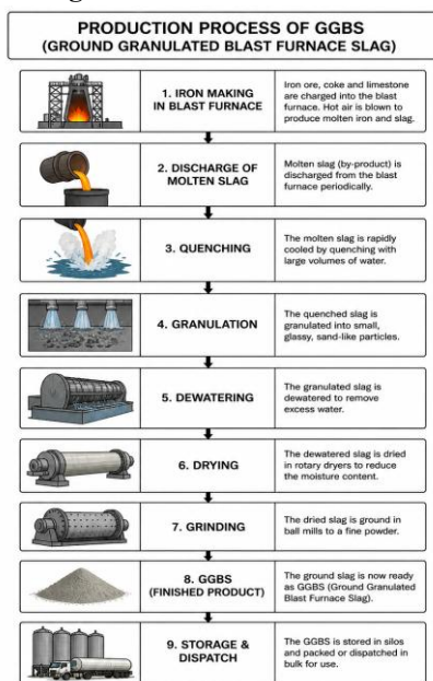
Fig 3.X: Flow Chart of Production Process of GGBS
