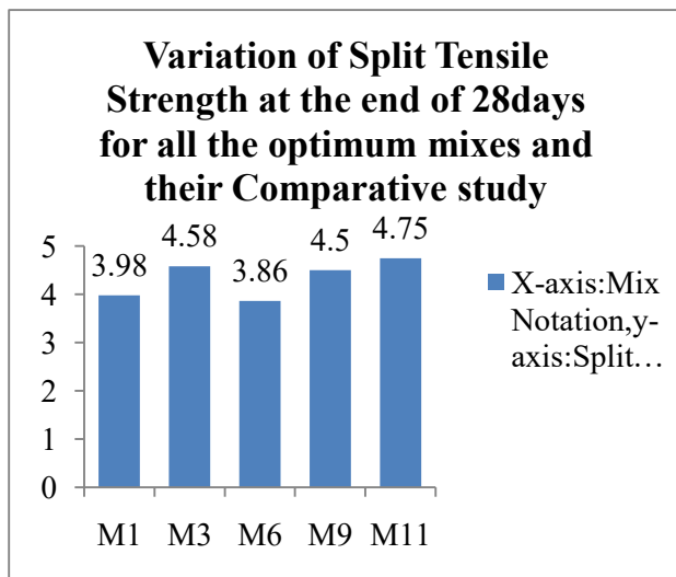
Graph 4.14: Variation of Split Tensile at the end of 28days for all the optimum mixes and their Comparative study
