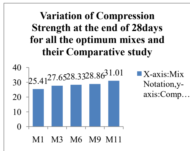
Graph 4.13: Variation of Compression Strength at the end of 28days for all the optimum mixes and their Comparative study
