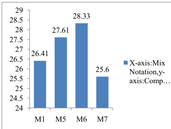
Graphs 4.5: Variation of Compression strength with fixed Ground Granulated Blast Furnace Slag (GGBS) %(10%) vs. variation of carbon fiber %.at the end of 7days
