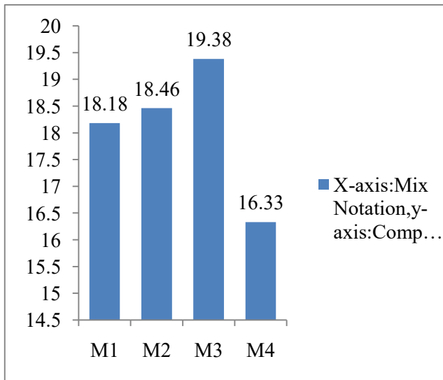
Graph 4.1: Variation of Compression strength with variation of Ground Granulated Blast Furnace Slag (GGBS) %at the end of 7days
