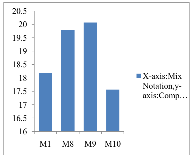
Graphs 4.5: Variation of Compression strength with fixed Ground Granulated Blast Furnace Slag (GGBS) %(10%) vs. variation of carbon fiber %.at the end of 7days
