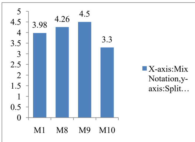
Graph 4.12 Variation of Split tensile strength with fixed Ground Granulated Blast Furnace Slag (GGBS) % (10%) + Carbon fiber% (1%) + Steel fibre% (1%) at the end of 28days
