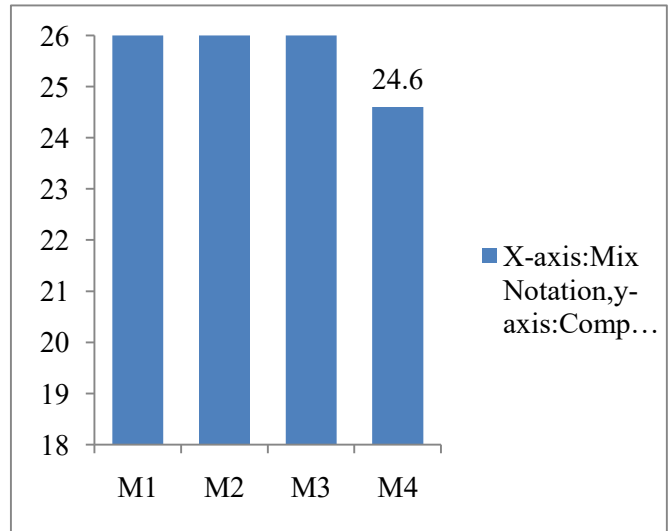
Graph 4.2: Variation of Compression strength with variation of Ground Granulated Blast Furnace Slag (GGBS) %at the end of 28days
