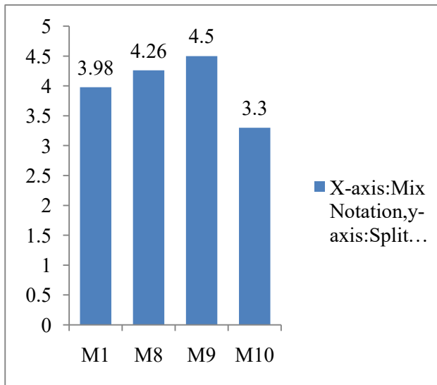
Graph 4.11: Variation of Split tensile strength with fixed Ground Granulated Blast Furnace Slag (GGBS) %(10%) vs variation of Carbon fibers % at the end of 28days
