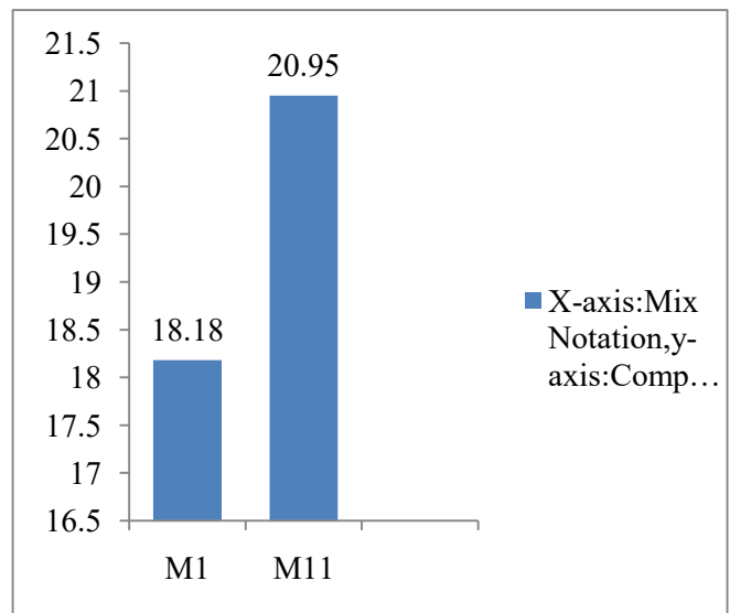
Graph 4.7: Variation of Compression strength with fixed Ground Granulated Blast Furnace Slag (GGBS) % (10%) + Carbon fiber% (1%) + Steel fibre% (1%) at the end of 7days
