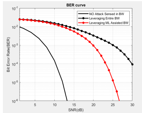
Fig.7 Error Rates for Different Conditions
