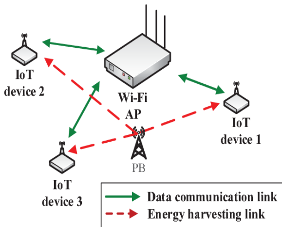
Fig.1 Typical Energy Harvesting at Hub of IoT Network
