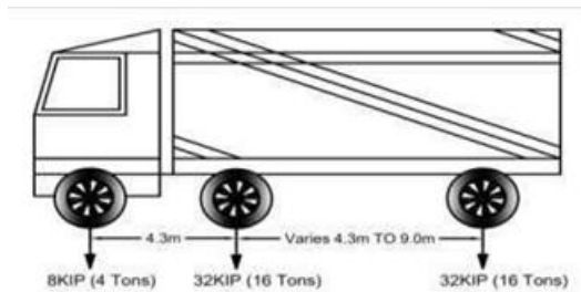
FIG 4. HS20-44 DESIGN TRUCK
