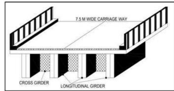
FIG. 1. TYPICAL SECTION OF T- BEAM BRIDGE
