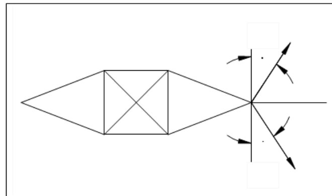
Figure 5: Conductor tension due to line deviation
