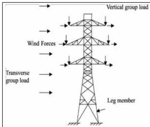
Figure 1: A suspension lattice steel tower resist combination loading from transverse and vertical directions [5].
