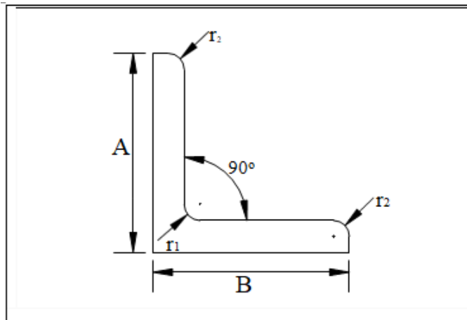
Figure 2: L-section bar used to form a tower structure.
