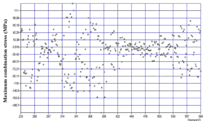
Figure 10: Maximum combination stress for middle conductor and bottom conductor broken.
