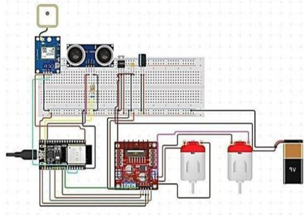
Fig.3.1.2. Circuit Diagram
