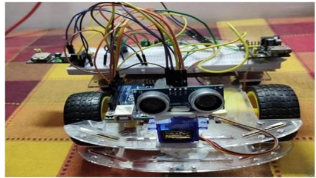
Fig.3.1.1. Design of the robot
