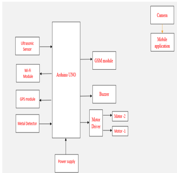
Fig.4.1.Block Diagram
