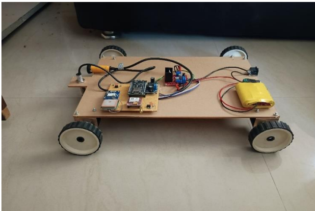
Fig.6.3.Side View of the Multipurpose Military Robot with Electronics and Power System
