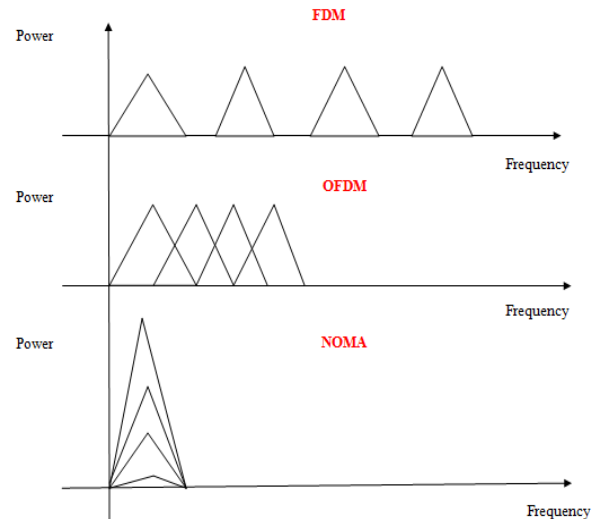
Fig.1 Comparative Spectra of FDM, OFDM and NOMA
