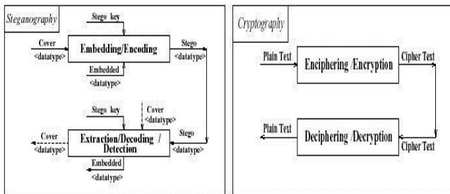
Fig. 1: Steganography versus Cryptography
