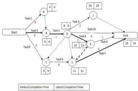
Fig 8: Tree Diagram For CPM Method
