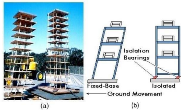
Fig 1.6. Base Isolation
