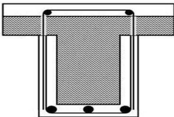
Fig 1.5. Beam Jacketing
