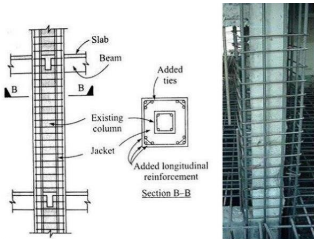
Fig 1.4. Column Jacketing
