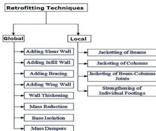
Fig 1.1 Retrofitting Techniques
