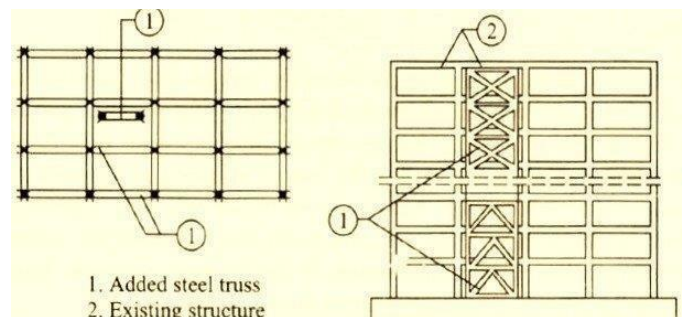
Fig 1.3. RC Building retrofitted by steel bracing
