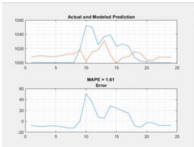
Fig. 2. Forecasted and Actual Yield.
