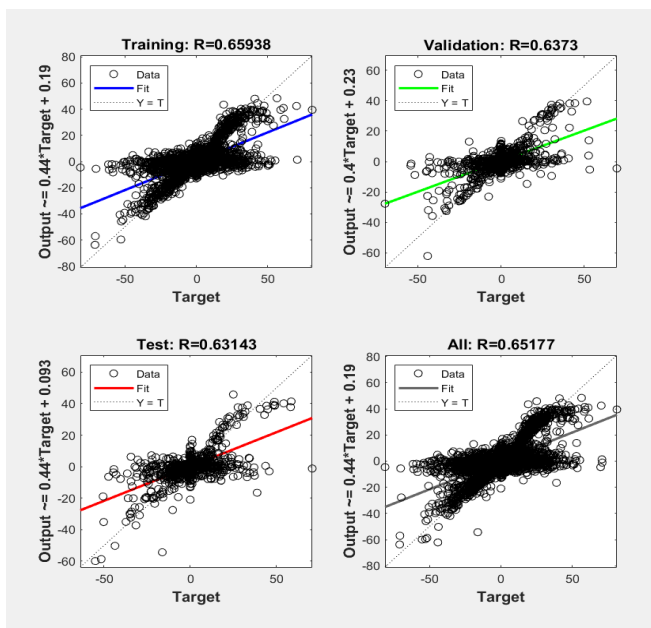
Fig. 3. Regression Analysis of Forecasting.
