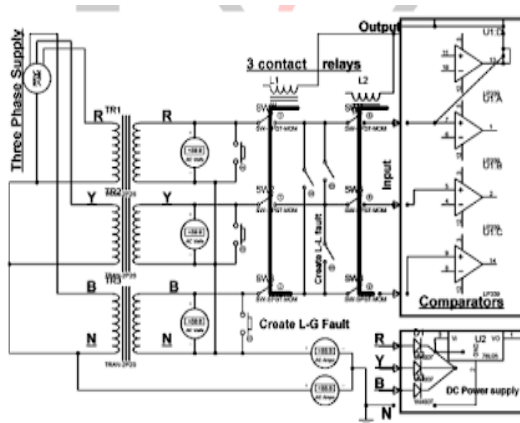
Fig -2: Three Phase Fault Analysis Circuit Diagram
