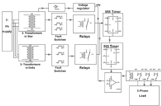
Fig -1: Three Phase Fault Analysis Block Diagram
