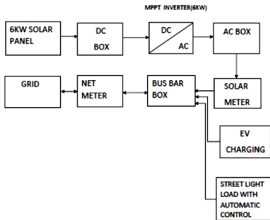
Fig. 2: Block diagram of PV plant
