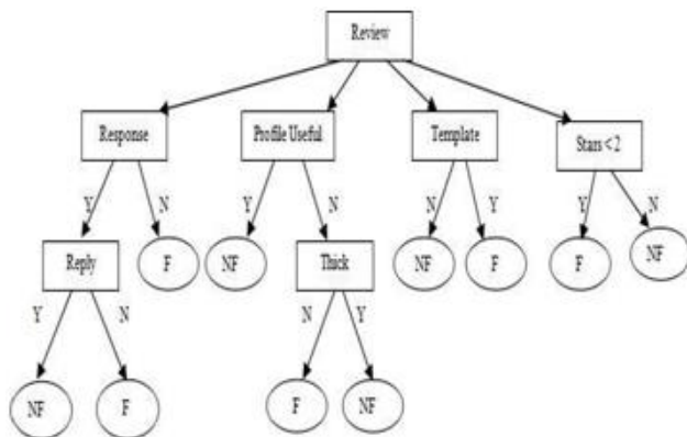
Fig 2: Decision Rule classifier tree.
