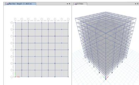
Figure 2 - Plan and 3D view of bare frame Building of G+12 stories building
