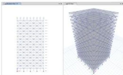
Figure 7 - 3D View and Elevation of 2 story diagrid structure of G+18 stories building
