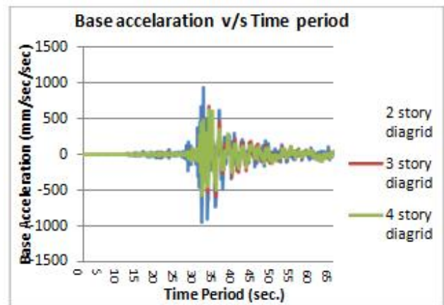
Figure 15 - Base Acceleration due to Time History analysis in G+18 storied Building
