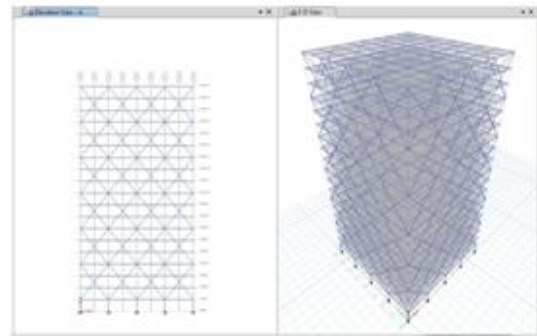
Figure 8 - View and Elevation of 3 story diagrid structure of G+18 stories building
