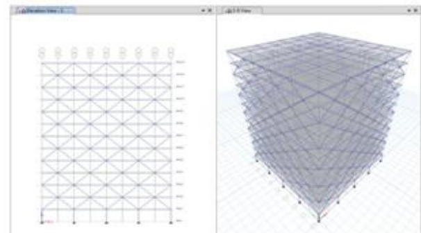
Figure 3 - 3D View and Elevation of 2 story diagrid structure of G+12 stories building
