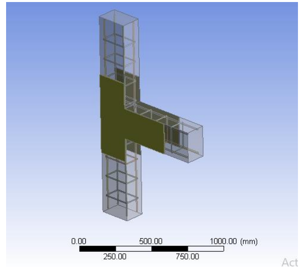
Fig 11: Side wrapping model
