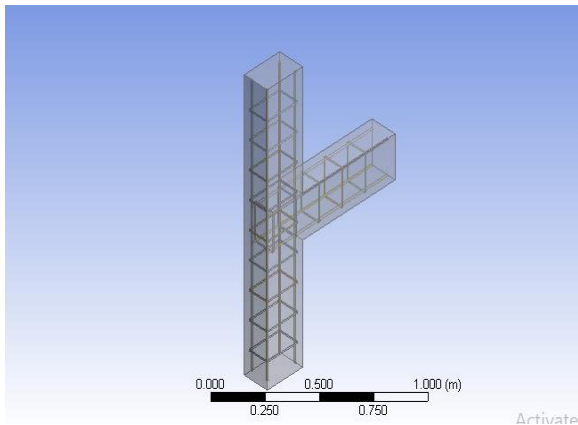
Fig 9: No wrapping model
