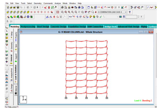
Fig 6: Bending Moment Of Beams In STAAD Pro
