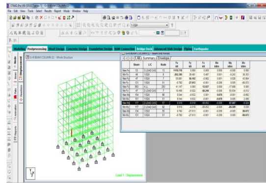
Fig 5: Reactions
