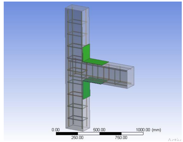
Fig 12: Top-bottom wrapping model
