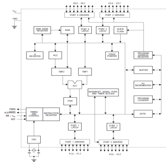
Block Diagram of AT89C52
