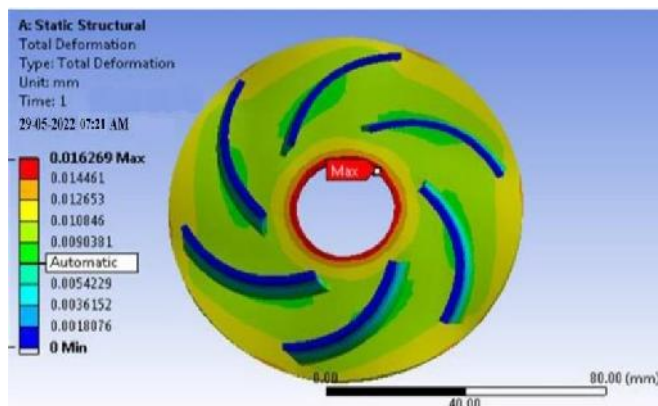
Figure No 4.3: Total deformation of CFRP material
