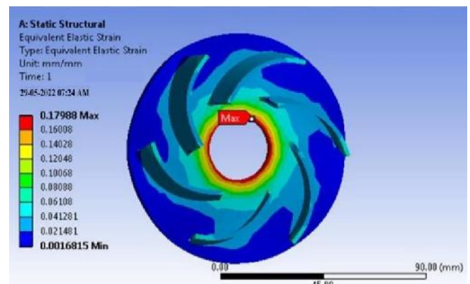
Figure No 4.5: Strain of GFRP material
