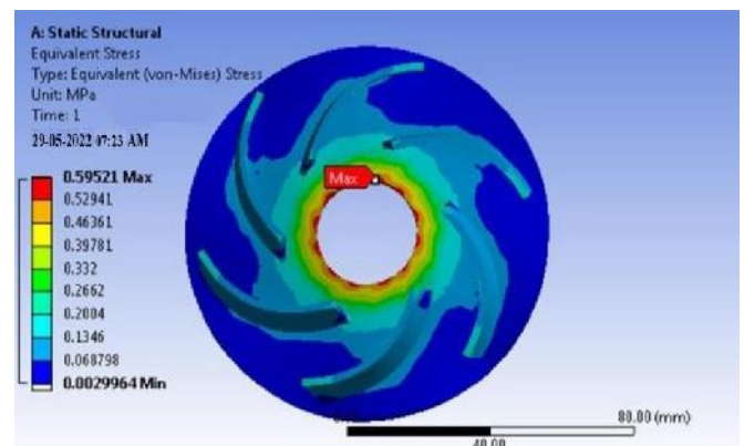
Figure No 4.4: Von-mises stress of GFRP material
