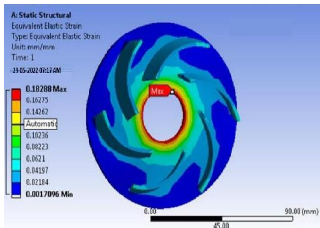
Figure No 4.2: Strain of CFRP material
