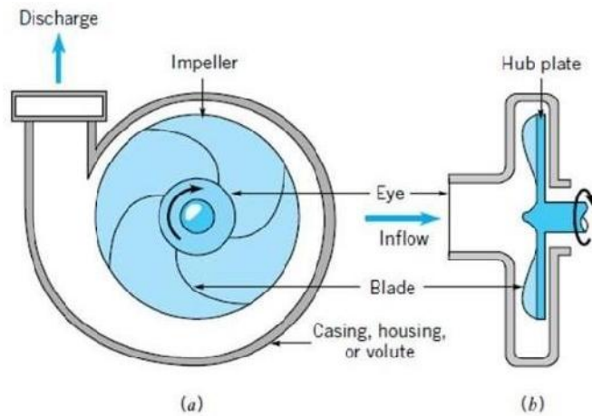
Figure No 1.1: Centrifugal pump basic working.
