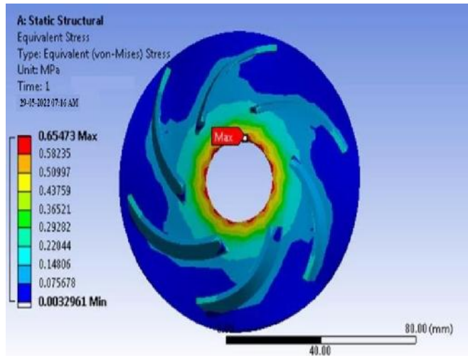
Figure No 4.1: Von-mises stress of CFRP material
