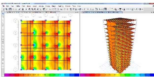
Fig 3. Stresses on building due to dynamic analysis
