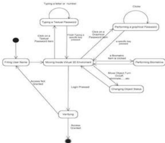
Fig.3:- state diagram of creating 3D password [1] [6] [7].
