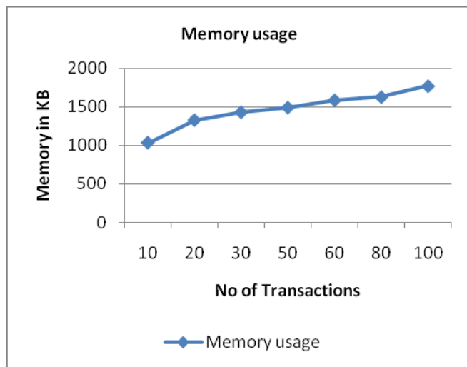
Figure 3.2 memory usage
