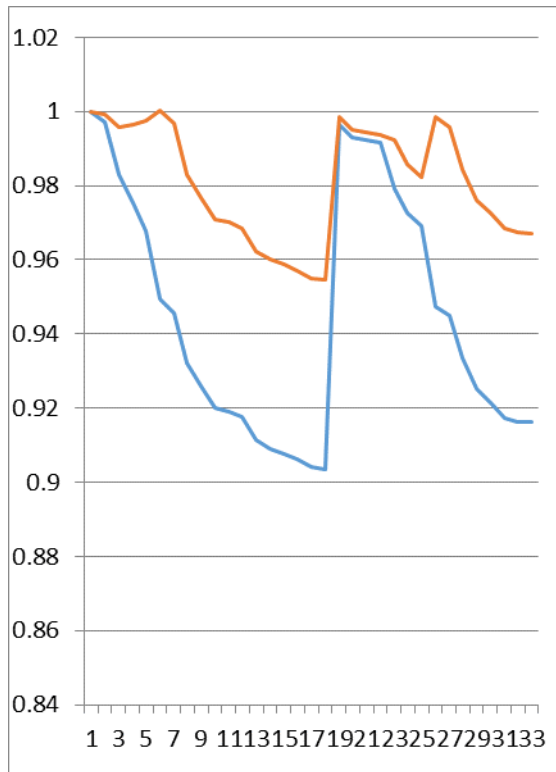
Fig. 2 Voltage profile comparison of IEEE 33 bus system with and with out DG
