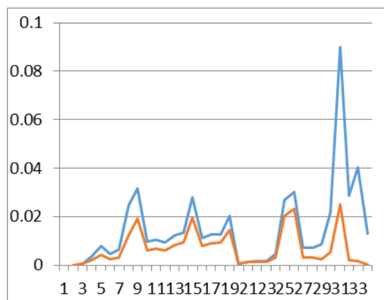
Fig 3 Comparison of Real power losses with and without DG
