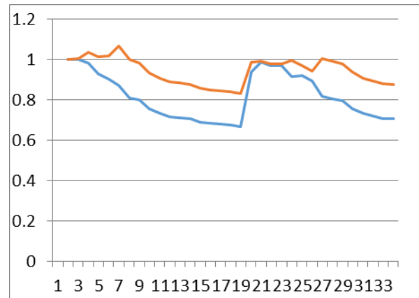
Fig 10 Comparison of Voltage Stability Index with and without DG
