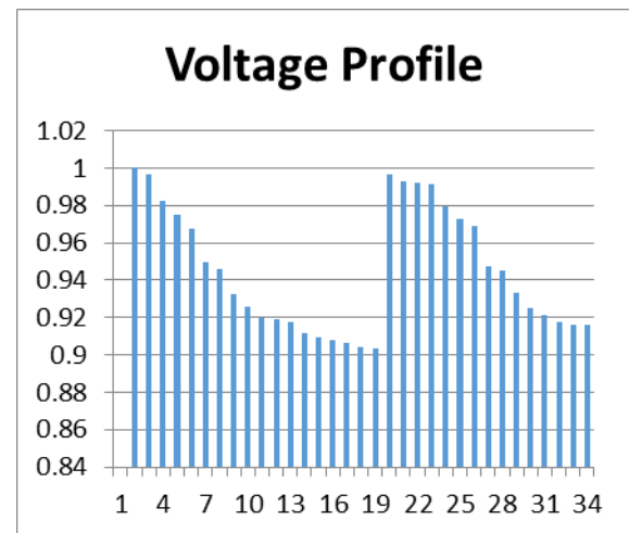
Fig. 2 Voltage profile Of IEEE 33 Bus system
