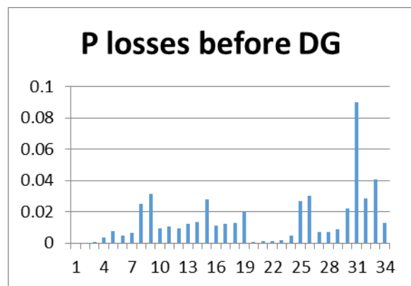
Fig. 3 Real power Losses before DG placement
