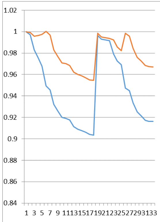
Fig. 8 Voltage profile comparison of IEEE 33 bus system with and with out DG
