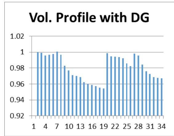
Fig. 5 Voltage Profile of IEEE 33 Bus system after placing DG
