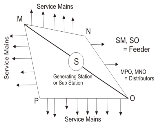
Fig.1 Distribution System
