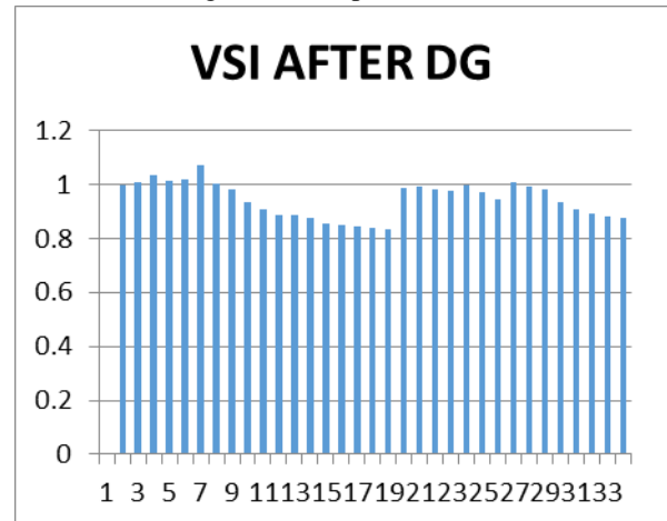
Fig 7 Voltage Stability Index With DG of IEEE 33 bus system
