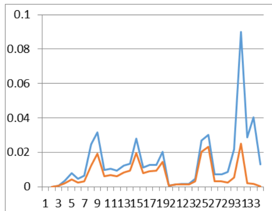
Fig 9 Comparison of Real power losses with and without DG
