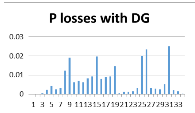
Fig. 6 Real Power losses with DG placement in IEEE 33 bus system
