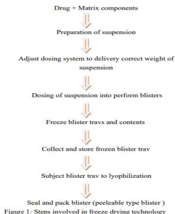
Figure 1: Steps involved in freeze drying technology
