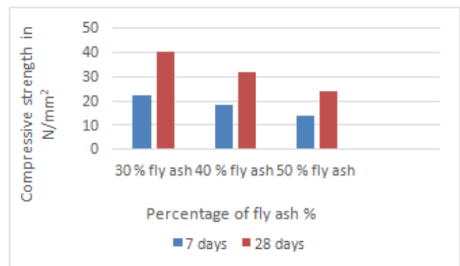
Figure 1 Compressive strength for M30
