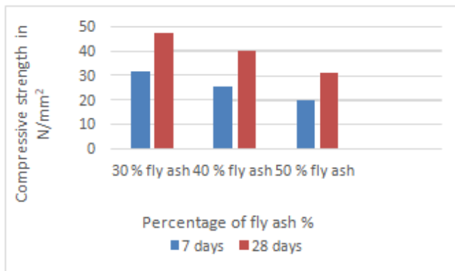
Figure 2 Compressive strength for M40
