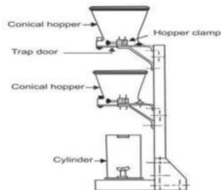
Apparatus for compaction factor
