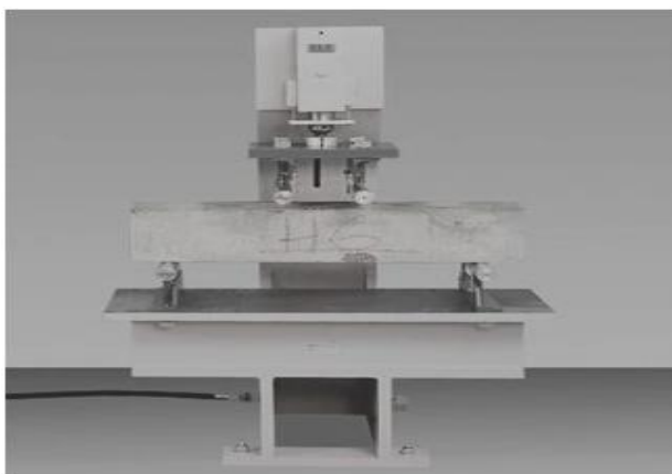
Flexural test machine
