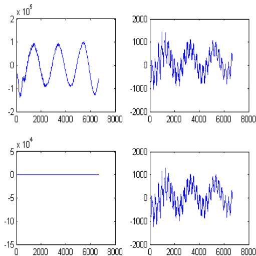
Fig. 10 Fault detection for Single line to ground fault in phase A
