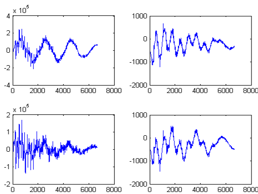
Fig: 9 angle Line Phase B and C fault detection
