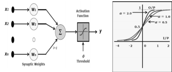
Fig: 2 A single neuron and sigmoidal activation
