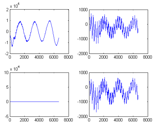
Fig. 11 Fault detection for Single line to ground fault in phase C
