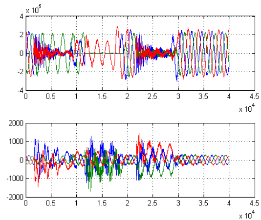
Fig: 6 Shows the current waveform of Ground to Line
