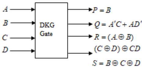
Figure 6: DKG Gate
