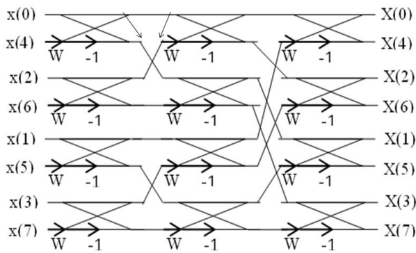
Figure 9: Flow Diagram of FFT using Folding Technique
