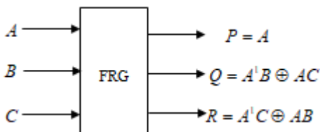
Figure 2: Fredkin gate
