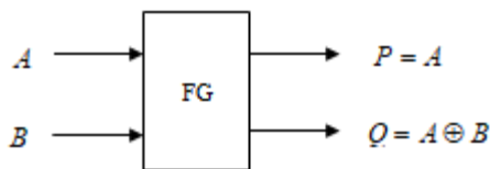
Figure 1: Feynman gate
