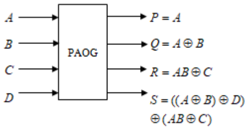
Figure 5: Block Diagram of the PAOG
