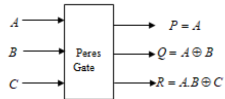
Figure 3: Peres gate
