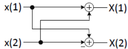
Figure 8: Radix-2 Butterfly
