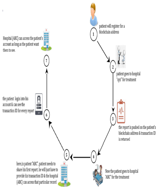
Figure 1:Architecture Diagram
