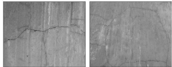
Fig.1.1 Case of break occurrence within the LMC bridge deck pavement
