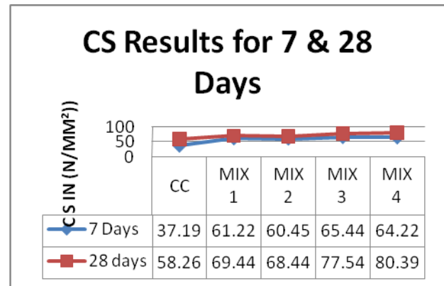
Graph:2 Shows 7 & 28 days C T results with various mixes of Latex
