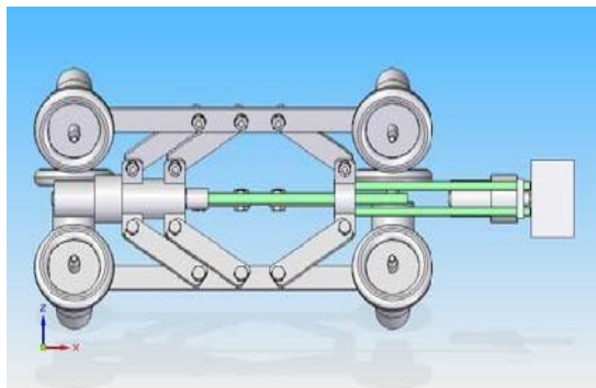
Fig.3: Assembly-Front view
