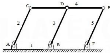
Fig.1: Simple Parallelogram Mechanism
