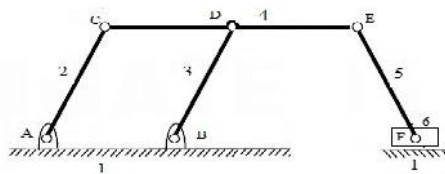
Fig.2: Modified Mechanism
