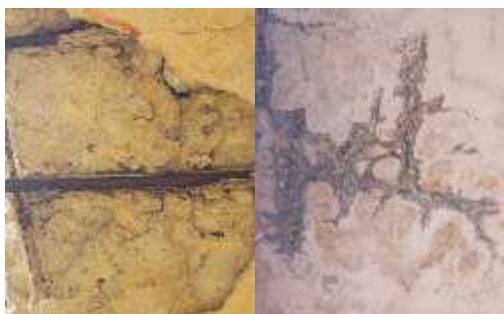
Fig3. Some areas detected during visual inspection which need immediate repair due to corrosion of steel reinforcements.
