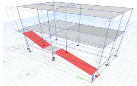
Fig.4: Planned View of Etabs Model 3D View of Etabs
