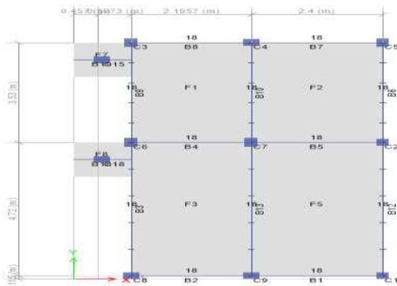
Fig.4:Planned View of Etabs Model
