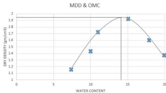
Graph 4.5.2 MDD = 1.92 gm./cm 3 & OMC = 14.70%
