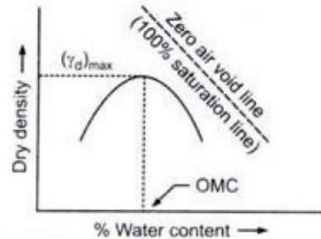
Fig : E Graph for MDD, OMC % 100% Saturation Line
