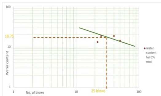
Liquid Limit Graph 4.3.A For 0% Root
