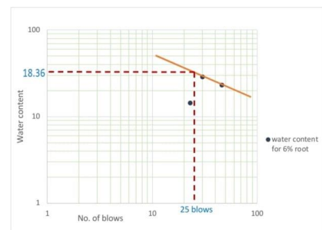
Liquid Limit Graph 4.3.D For 6% Root
