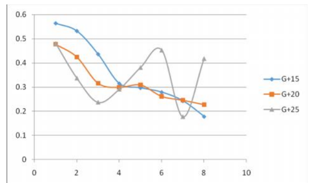
Chart. Storey drift graph for Rcc bare frames in X direction for KOYNA
