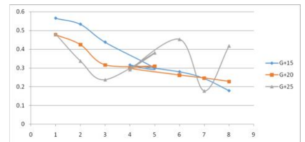
Chart. Storey drift graph for Rcc bare frames in Y direction for KOYNA.
