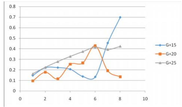
Chart. Storey drift graph for Rcc bare frames in Y direction for BHUJ
