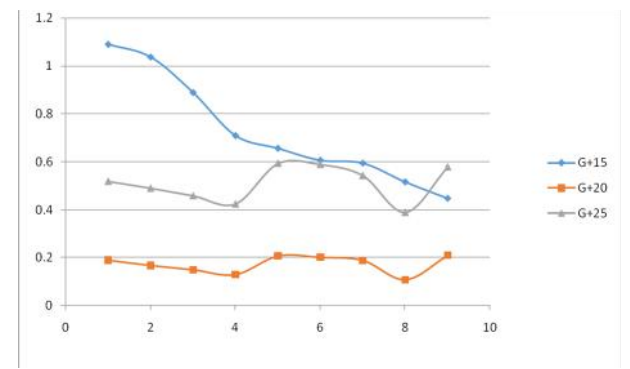
Chart. Storey drift graph for Rcc bare frames in X direction for BHUJ
