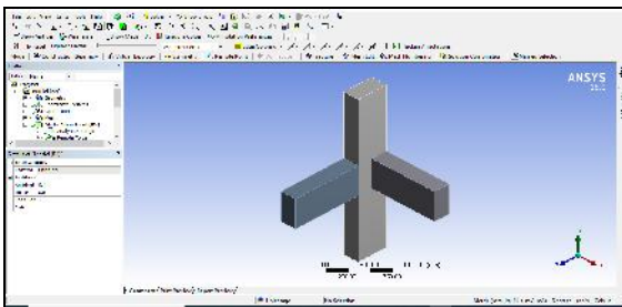
Fig 5 RCC Beam Column
