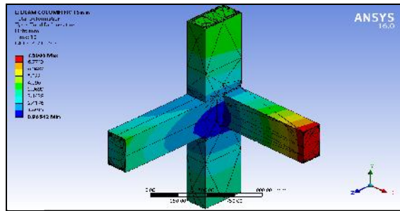
Fig 9 Deformation of NC15
