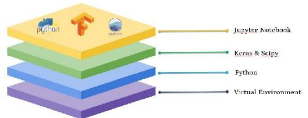
Fig 2. Technology Stack
