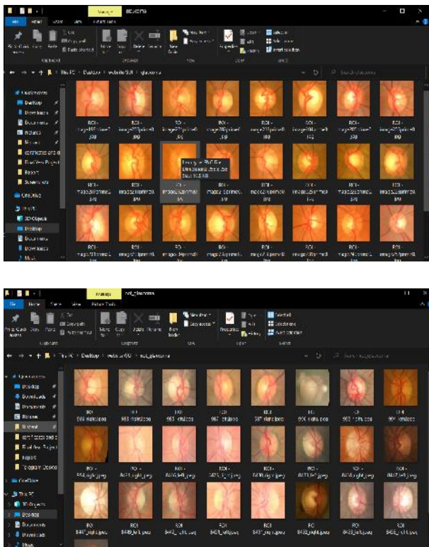
Fig 4. Dataset Images
