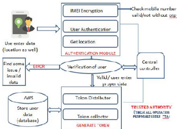
Figure 4: Proposed System architecture
