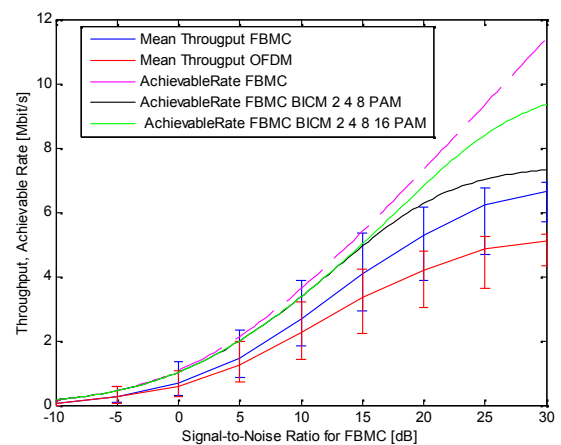
Fig.7. Throughput vs SNR
