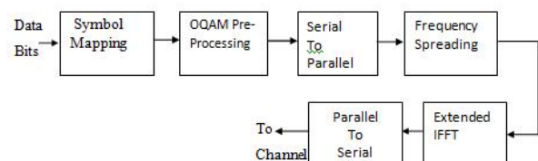
Fig.2 FBMC Transmitter
