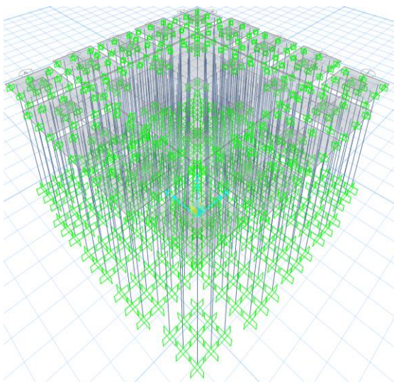
Fig 06: 3D model of Pile Foundation
