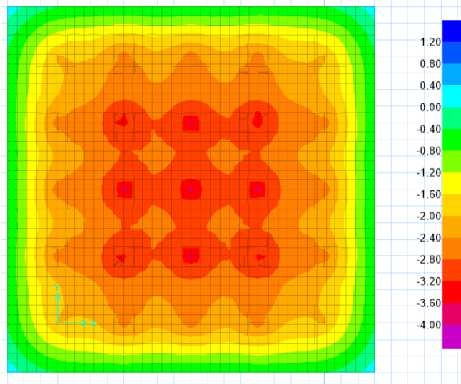
Fig 11: Pile Raft foundation Settlement
