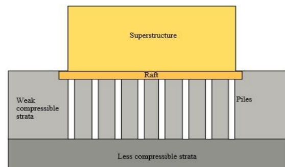
Fig 01: Piles with raft foundation.
