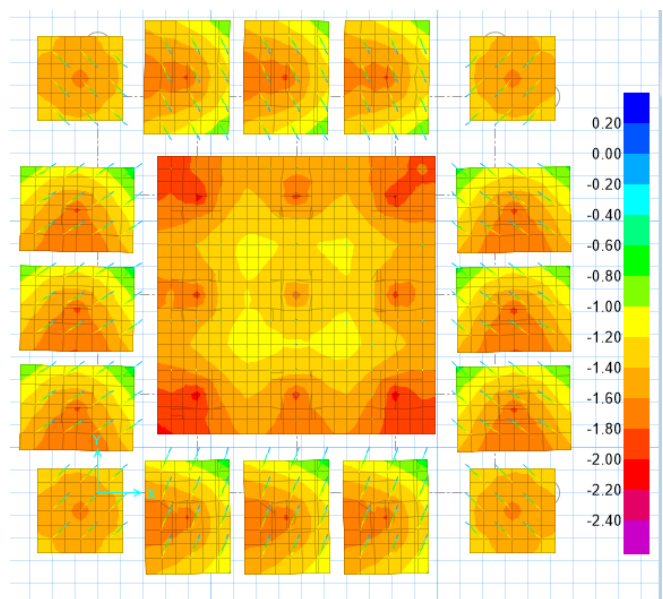
Fig 10: Pile foundation Settlement
