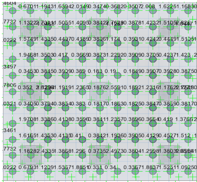
Fig 18: Pile foundation Punching Shear for 121 pile group
