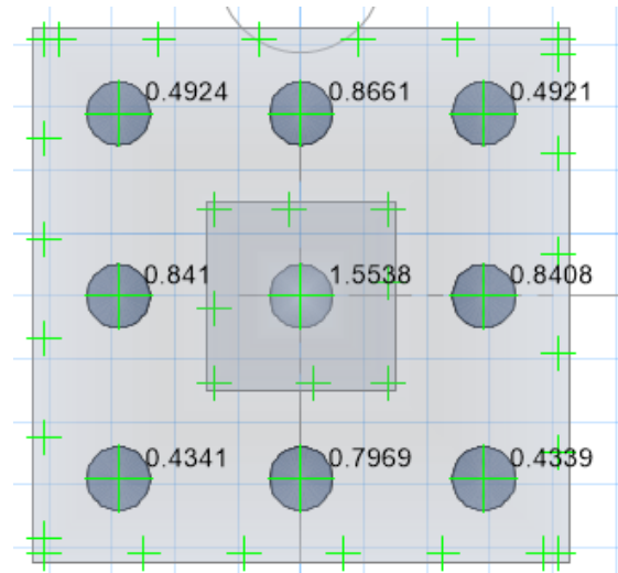
Fig 16: Pile foundation Punching Shear for 9 pile group.
