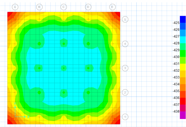
Fig 12: Raft foundation Soil Pressure Reaction
