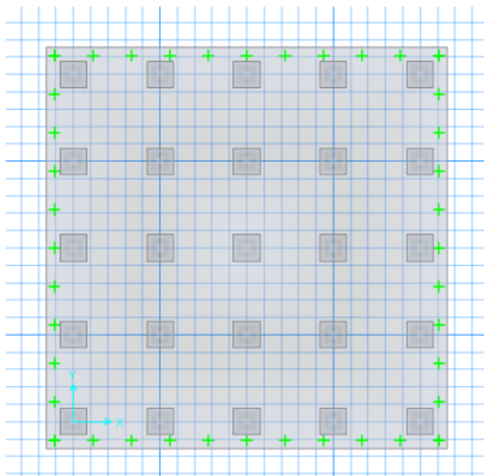
Fig 04: Finite Element Model of Raft Foundation
