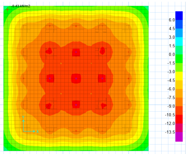
Fig 14: PileRaft foundation Soil Pressure Reaction
