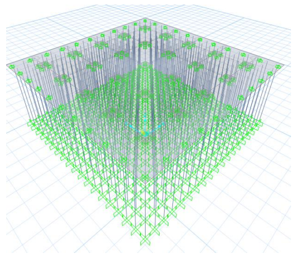
Fig 08: 3D model of Pile Raft Foundation
