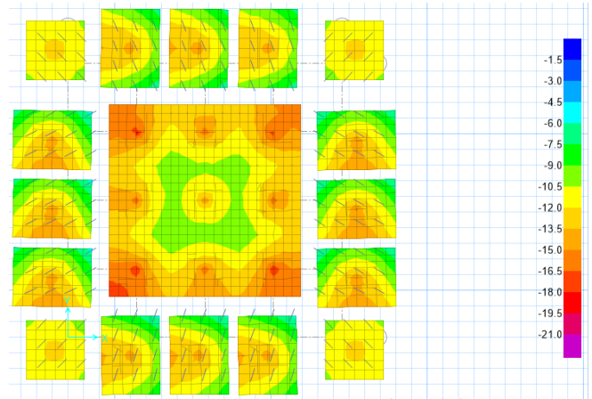
Fig 13: Pile foundation Soil Pressure Reaction
