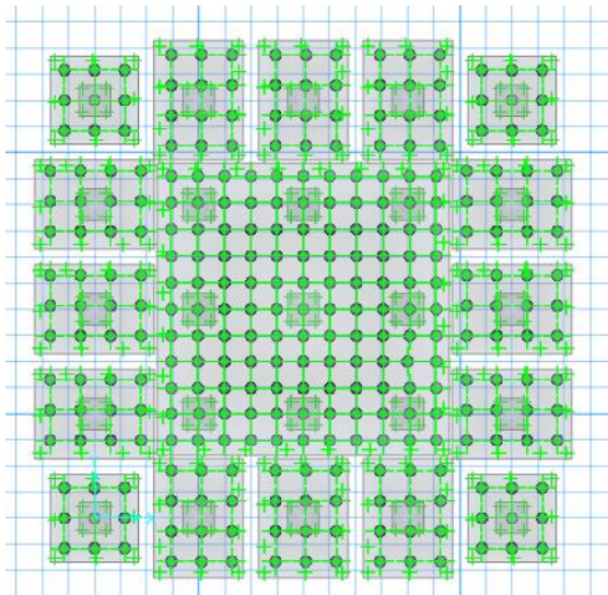
Fig 05: Finite Element Model of pile Foundation
