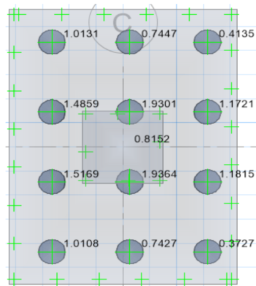
Fig 17: Pile foundation Punching Shear for 12 pile group
