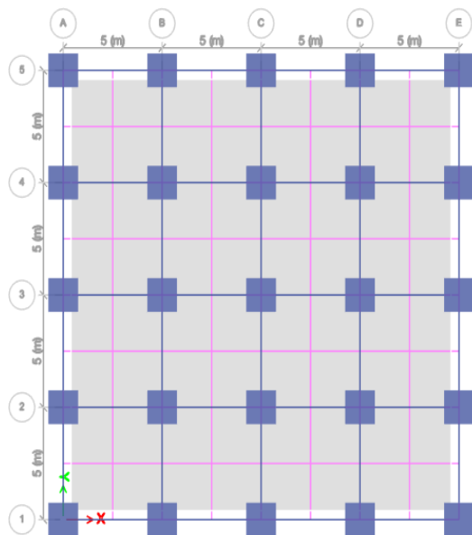
Fig 02: Plan Of structure.
