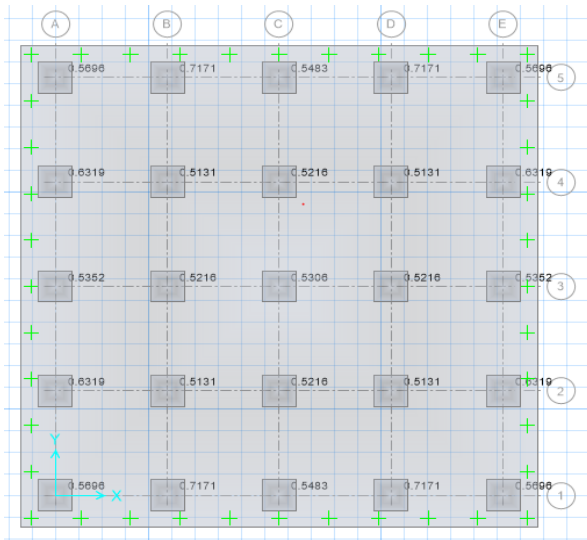
Fig 15: Raft foundation Punching Shear
