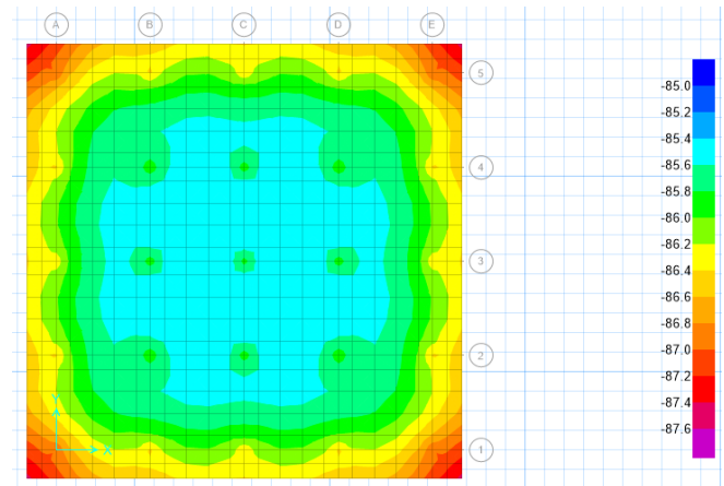
Fig 09: Raft foundation Settlement
