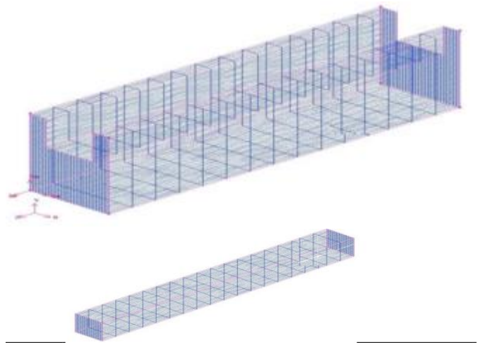
Figure 2.2 Meshing of the channel domain
