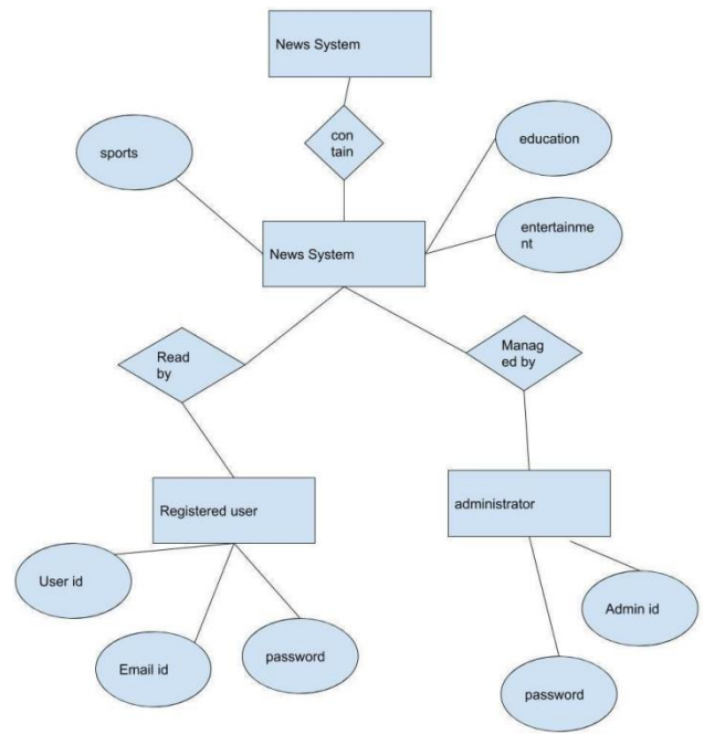
Entity-Relationship Diagram
