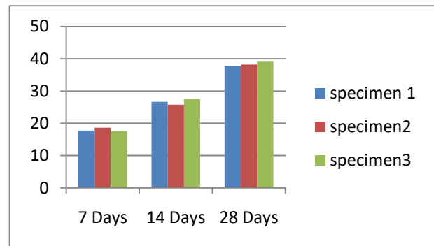
Graph COMPRESSIVE STRENGTH OF RHAC (10 %)
