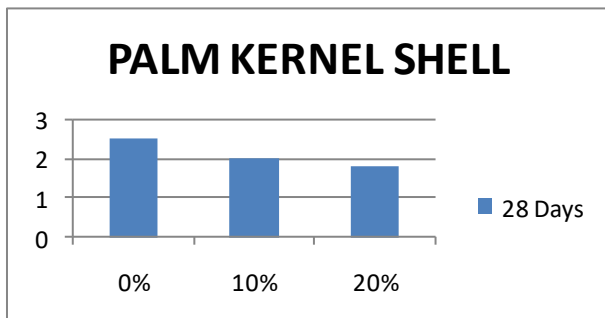
Comparison of Split Tensile strength of Palm Kernel Shell Concrete
