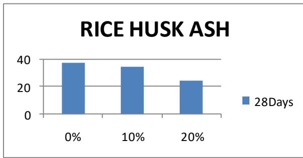
Comparison of Compressive strength of Rice Husk Ash
