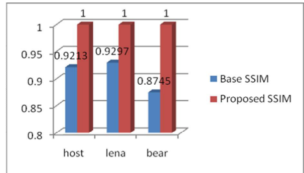
Fig 12. Graph Comparison of Base SSIM and ProposedSSIM.
