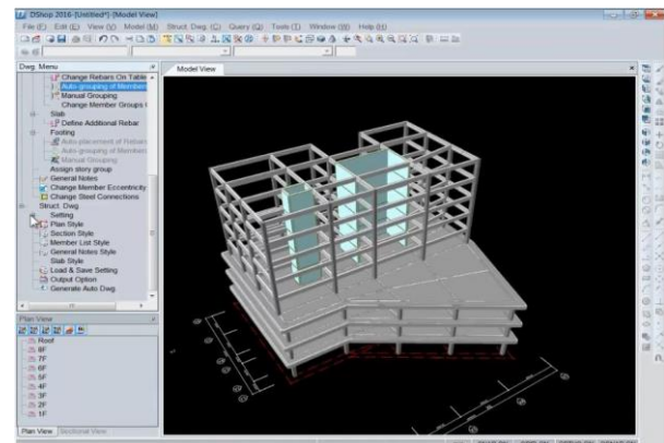
Fig 2 Making of structure using MIDAS
