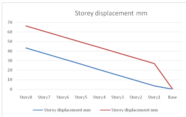
Fig 13: Displacement
