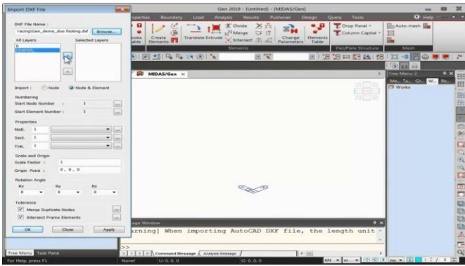
Fig 3: Importing DXF file
