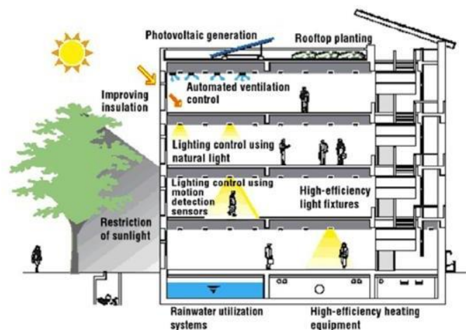
Fig. 3.1 Conceptual Drawing of Green Building
