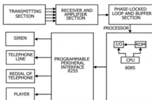
Fig.1-The block diagram of the “Self safety system for women security with vicinity tracking and SMS Alerting via GSM community”.
