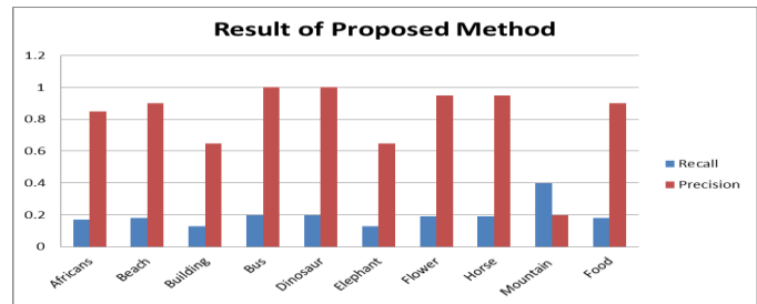
Figure 1.9: Graphical representation of Precision and Recall
