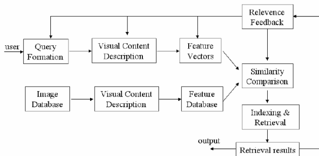
Figure 1.2 Content based image retrieval system
