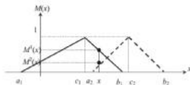
Fig.4. Building up the Fuzzy-Based Transformation Function
