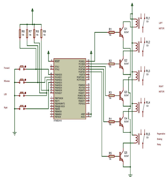
Fig2.1 operating relay
